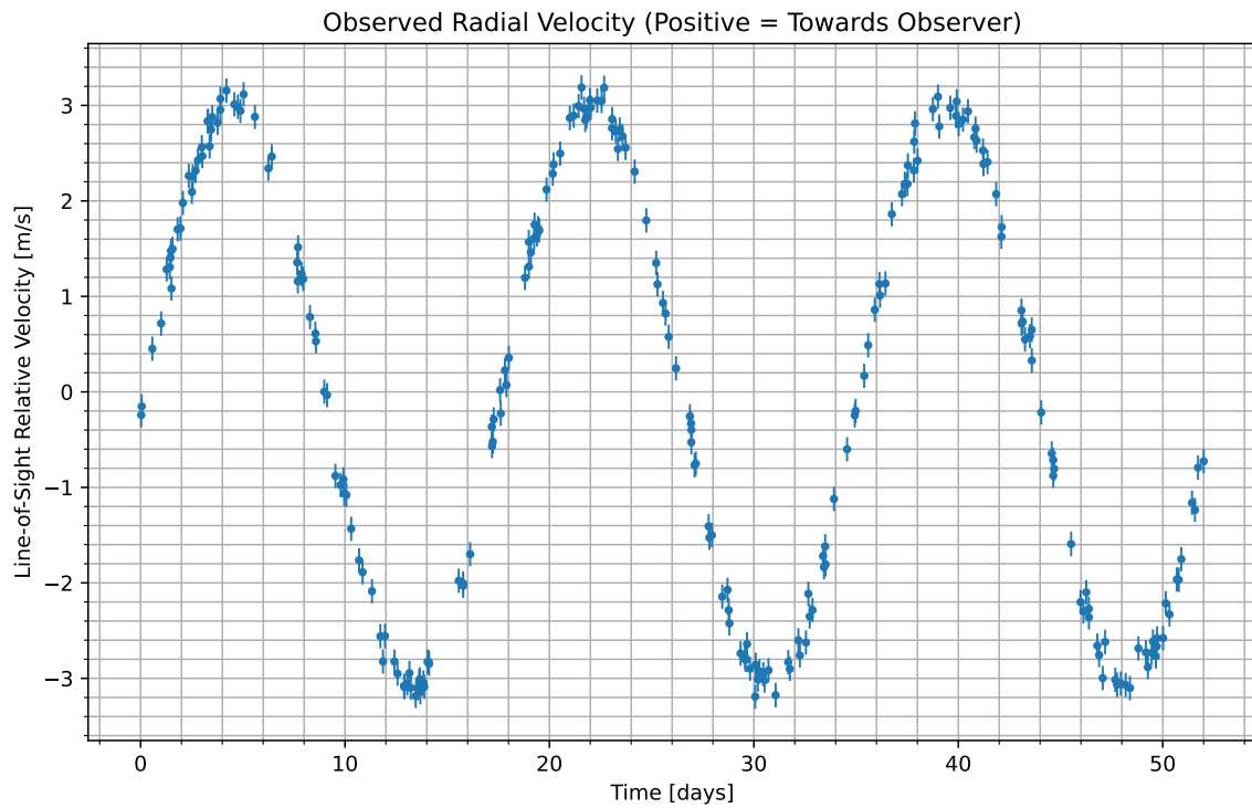
Figure 1: We have isolated the radial velocity of the host star due to the candidate planet. Data begins at UTC 2091-05-28/10:53. Positive values indicate the velocity at which the star is moving towards us; negative indicate the velocity at which it is moving away.
