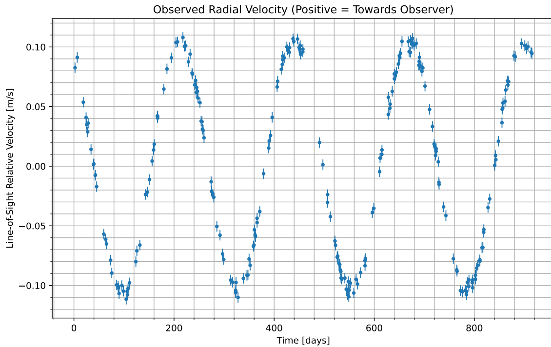
Figure 1: We have isolated the radial velocity of the host star due to the candidate planet. Data begins at UTC 2089-01-29/19:30. Positive values indicate the velocity at which the star is moving towards us; negative indicate the velocity at which it is moving away.
