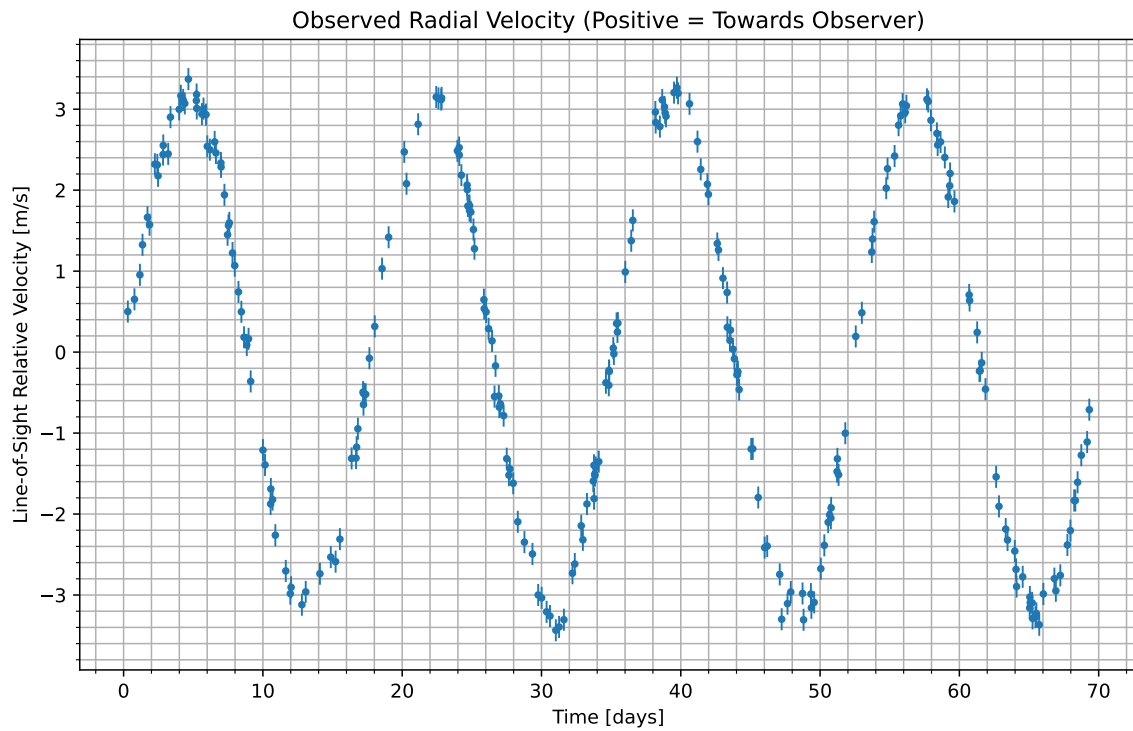
Figure 1: We have isolated the radial velocity of the host star due to the candidate planet. Data begins at UTC 2082-08-21/14:15. Positive values indicate the velocity at which the star is moving towards us; negative indicate the velocity at which it is moving away.
