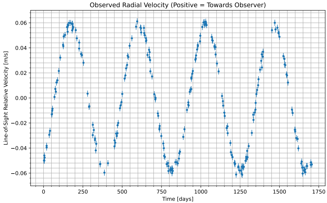
Figure 1: We have isolated the radial velocity of the host star due to the candidate planet. Data begins at UTC 2074-06-06/11:57. Positive values indicate the velocity at which the star is moving towards us; negative indicate the velocity at which it is moving away.
