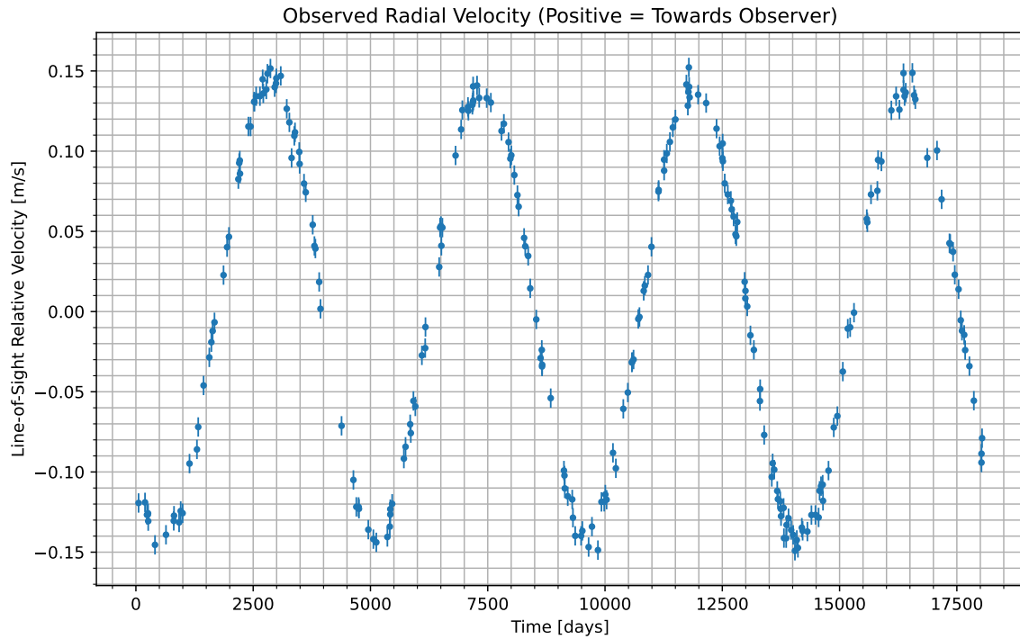
Figure 1: We have isolated the radial velocity of the host star due to the candidate planet. Data begins at UTC 2045-02-02/05:42. Positive values indicate the velocity at which the star is moving towards us; negative indicate the velocity at which it is moving away.
