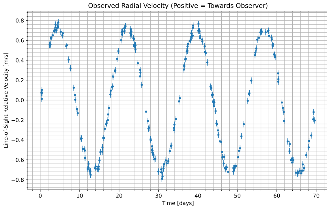
Figure 1: We have isolated the radial velocity of the host star due to the candidate planet. Data begins at UTC 2083-05-04/12:38. Positive values indicate the velocity at which the star is moving towards us; negative indicate the velocity at which it is moving away.
