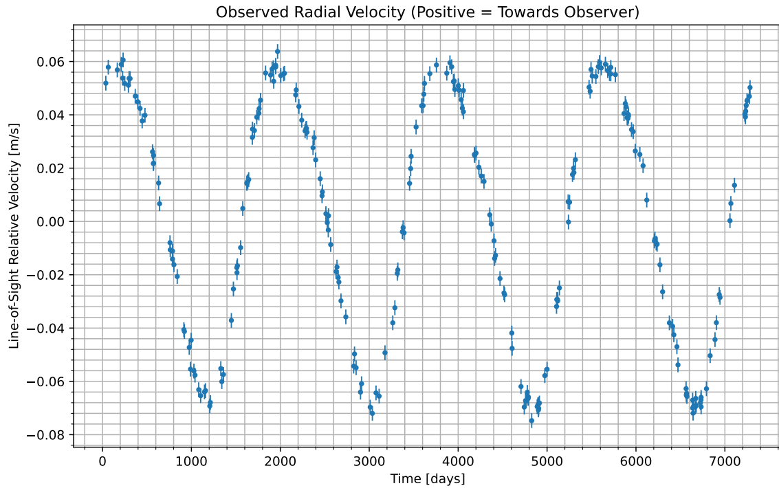
Figure 1: We have isolated the radial velocity of the host star due to the candidate planet. Data begins at UTC 2050-10-16/23:53. Positive values indicate the velocity at which the star is moving towards us; negative indicate the velocity at which it is moving away.
