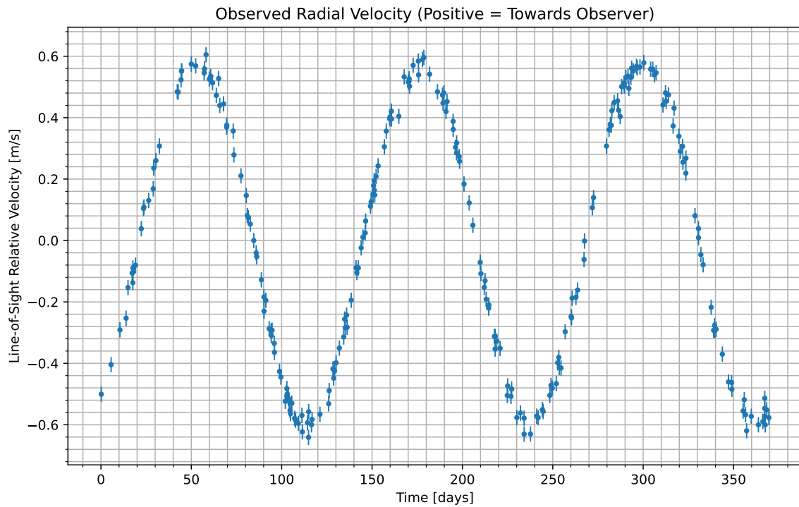
Figure 1: We have isolated the radial velocity of the host star due to the candidate planet. Data begins at UTC 2075-07-15/20:57. Positive values indicate the velocity at which the star is moving towards us; negative indicate the velocity at which it is moving away.
