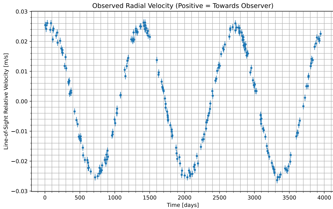
Figure 1: We have isolated the radial velocity of the host star due to the candidate planet. Data begins at UTC 2078-04-28/19:51. Positive values indicate the velocity at which the star is moving towards us; negative indicate the velocity at which it is moving away.
