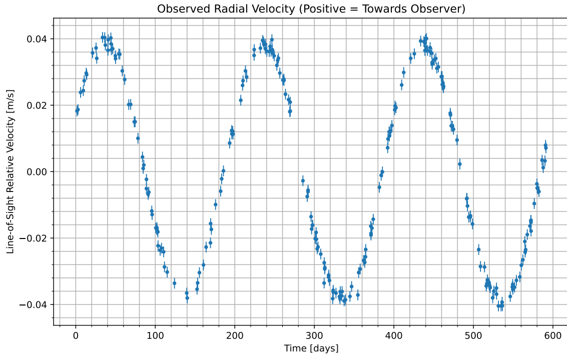
Figure 1: We have isolated the radial velocity of the host star due to the candidate planet. Data begins at UTC 2086-05-05/21:47. Positive values indicate the velocity at which the star is moving towards us; negative indicate the velocity at which it is moving away.
