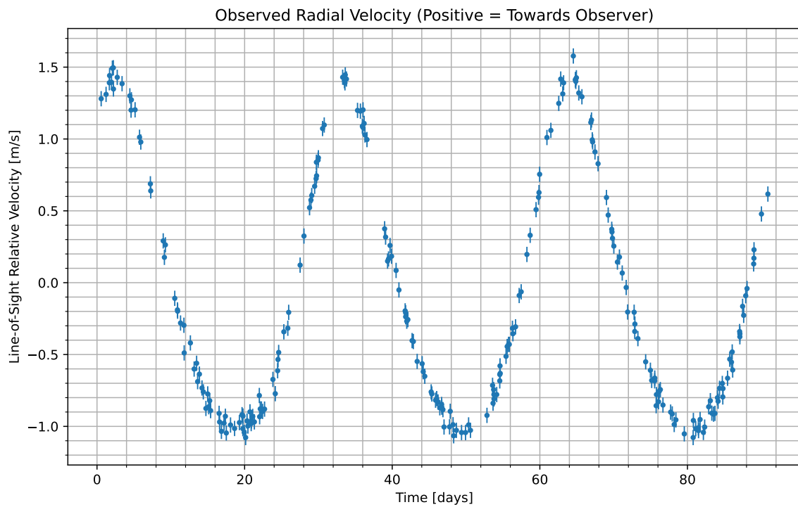
Figure 1: We have isolated the radial velocity of the host star due to the candidate planet. Data begins at UTC 2086-07-19/00:15. Positive values indicate the velocity at which the star is moving towards us; negative indicate the velocity at which it is moving away.
