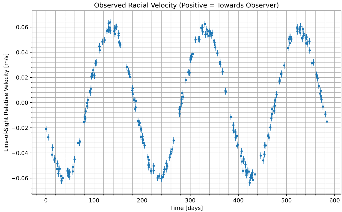
Figure 1: We have isolated the radial velocity of the host star due to the candidate planet. Data begins at UTC 2090-02-10/11:29. Positive values indicate the velocity at which the star is moving towards us; negative indicate the velocity at which it is moving away.
