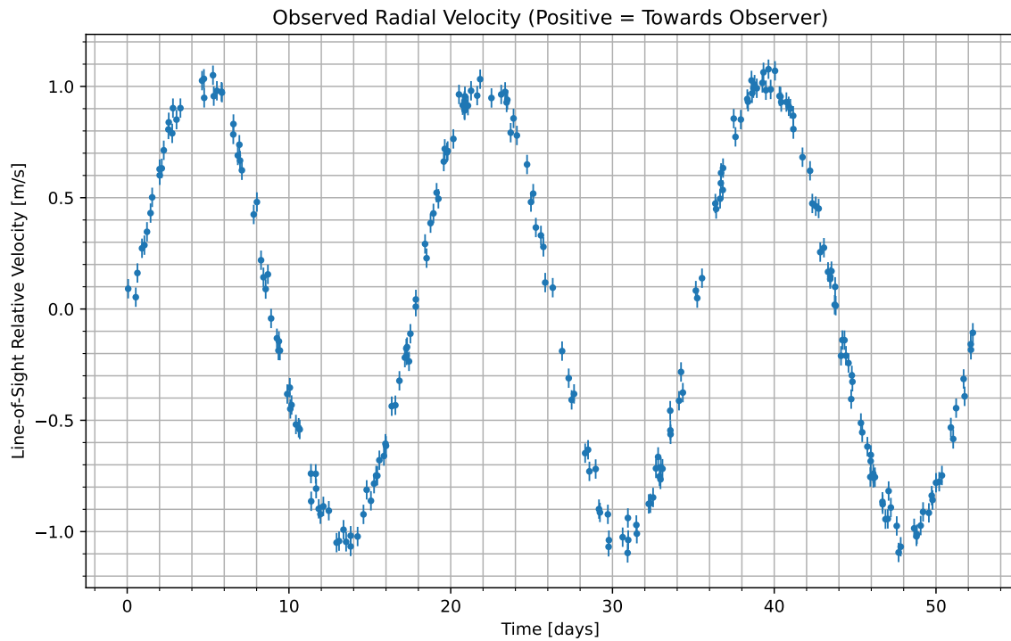
Figure 1: We have isolated the radial velocity of the host star due to the candidate planet. Data begins at UTC 2076-02-04/12:10. Positive values indicate the velocity at which the star is moving towards us; negative indicate the velocity at which it is moving away.
