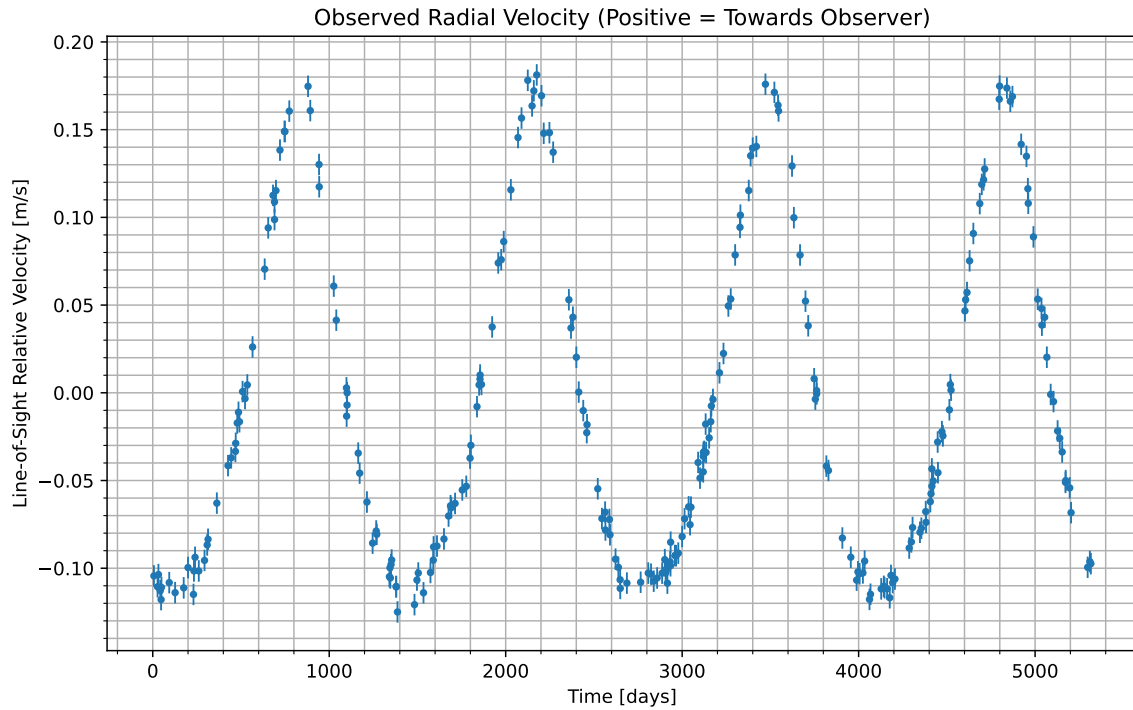
Figure 1: We have isolated the radial velocity of the host star due to the candidate planet. Data begins at UTC 2076-04-11/06:04. Positive values indicate the velocity at which the star is moving towards us; negative indicate the velocity at which it is moving away.
