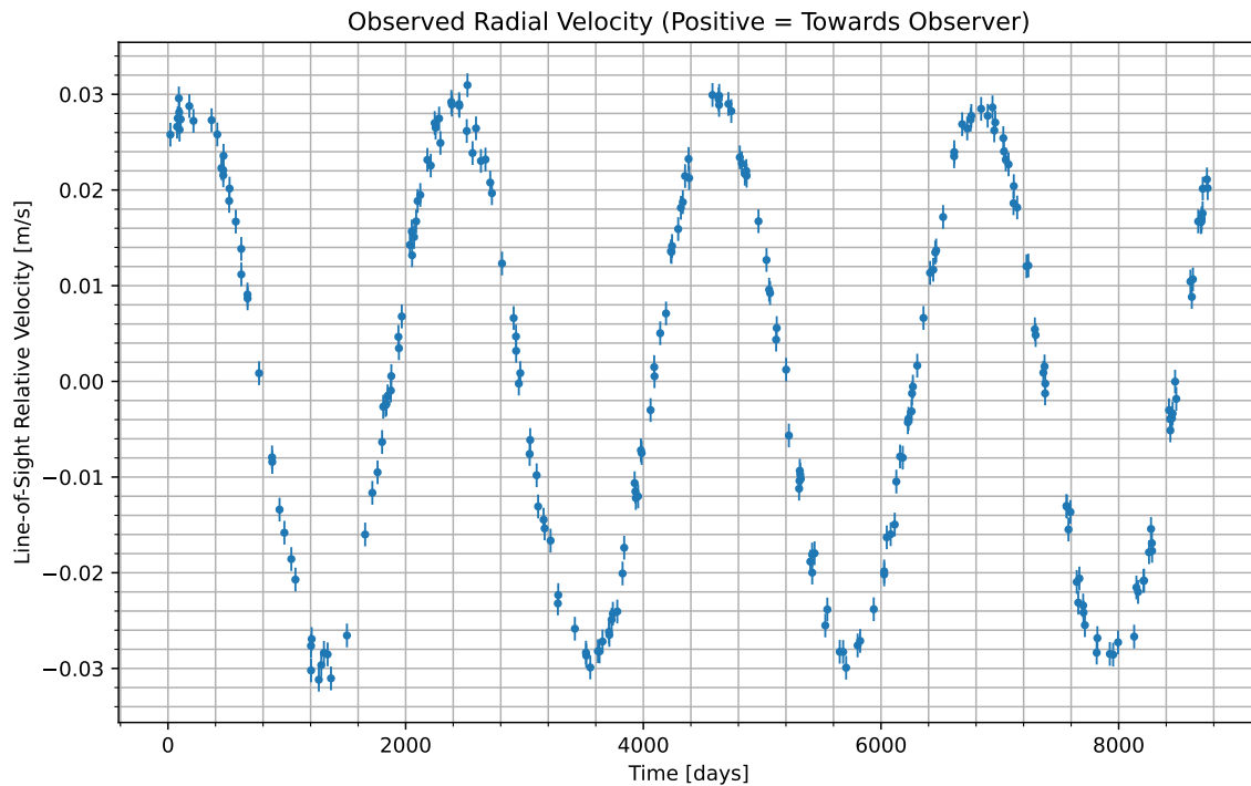
Figure 1: We have isolated the radial velocity of the host star due to the candidate planet. Data begins at UTC 2059-04-27/11:25. Positive values indicate the velocity at which the star is moving towards us; negative indicate the velocity at which it is moving away.
