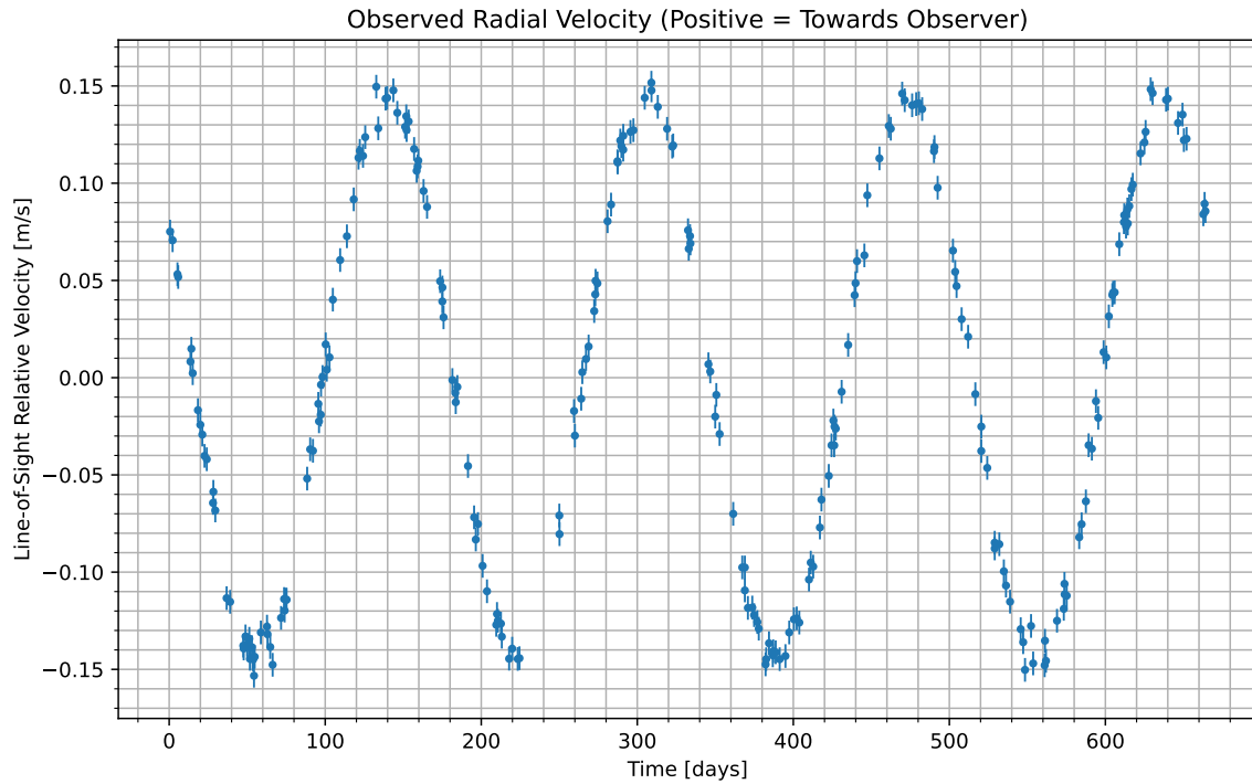
Figure 1: We have isolated the radial velocity of the host star due to the candidate planet. Data begins at UTC 2079-02-03/00:24. Positive values indicate the velocity at which the star is moving towards us; negative indicate the velocity at which it is moving away.
