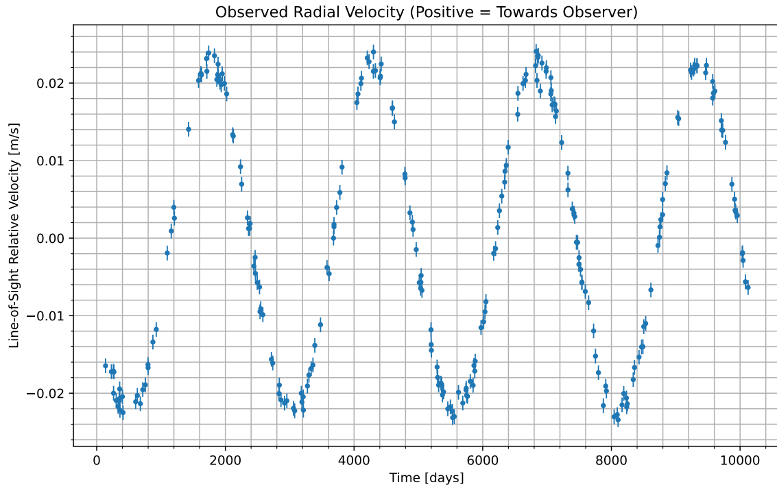
Figure 1: We have isolated the radial velocity of the host star due to the candidate planet. Data begins at UTC 2050-10-19/10:01. Positive values indicate the velocity at which the star is moving towards us; negative indicate the velocity at which it is moving away.
