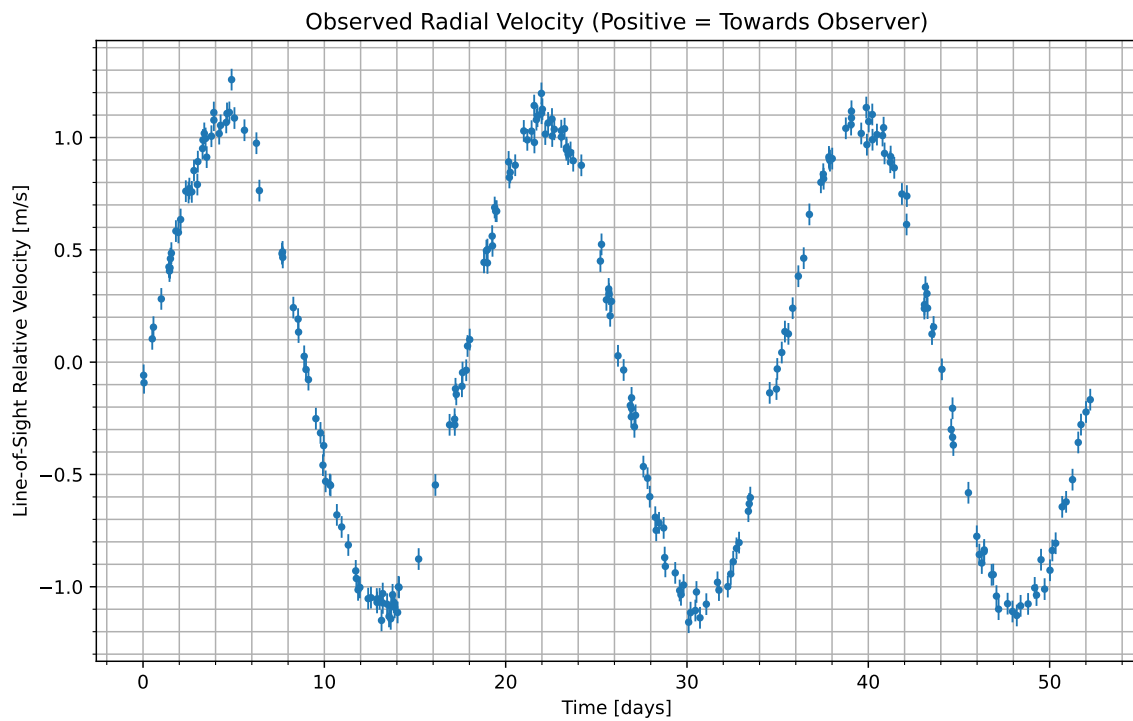
Figure 1: We have isolated the radial velocity of the host star due to the candidate planet. Data begins at UTC 2072-11-10/19:56. Positive values indicate the velocity at which the star is moving towards us; negative indicate the velocity at which it is moving away.
