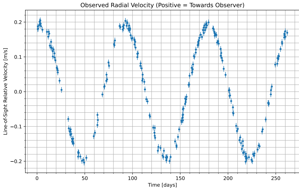
Figure 1: We have isolated the radial velocity of the host star due to the candidate planet. Data begins at UTC 2087-03-18/19:59. Positive values indicate the velocity at which the star is moving towards us; negative indicate the velocity at which it is moving away.
