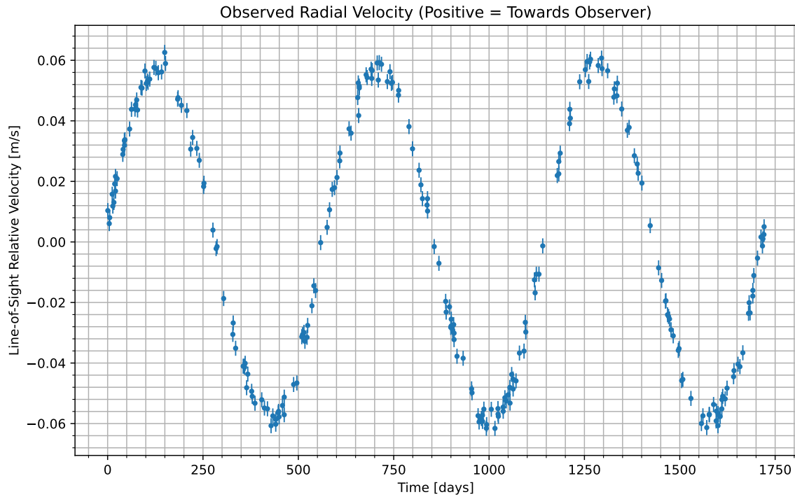
Figure 1: We have isolated the radial velocity of the host star due to the candidate planet. Data begins at UTC 2084-04-28/07:38. Positive values indicate the velocity at which the star is moving towards us; negative indicate the velocity at which it is moving away.
